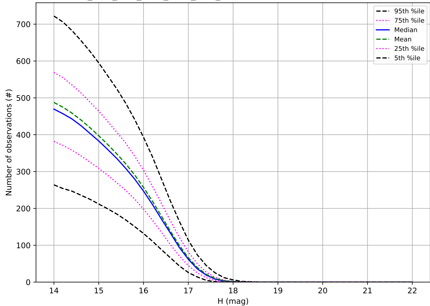
ddf_acor_sf10_lsf15_lsr50_v3.4_10yrs: Number of observations Trojan
