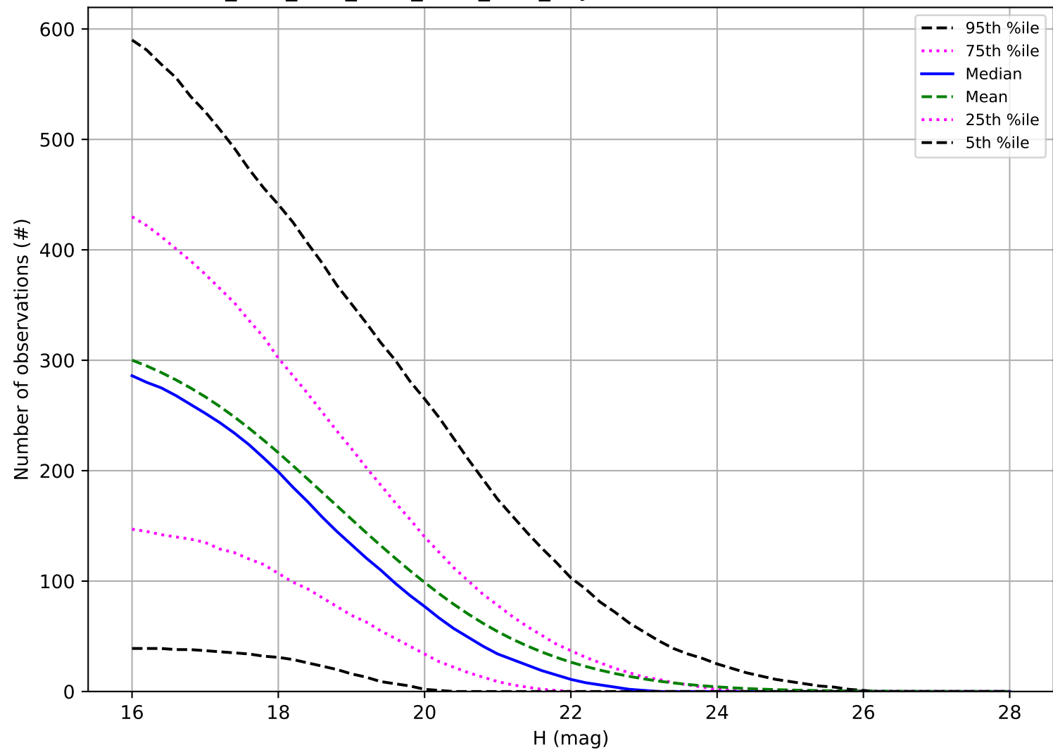
ddf_acor_sf10_lsf15_lsr50_v3.4_10yrs: Number of observations PHA
