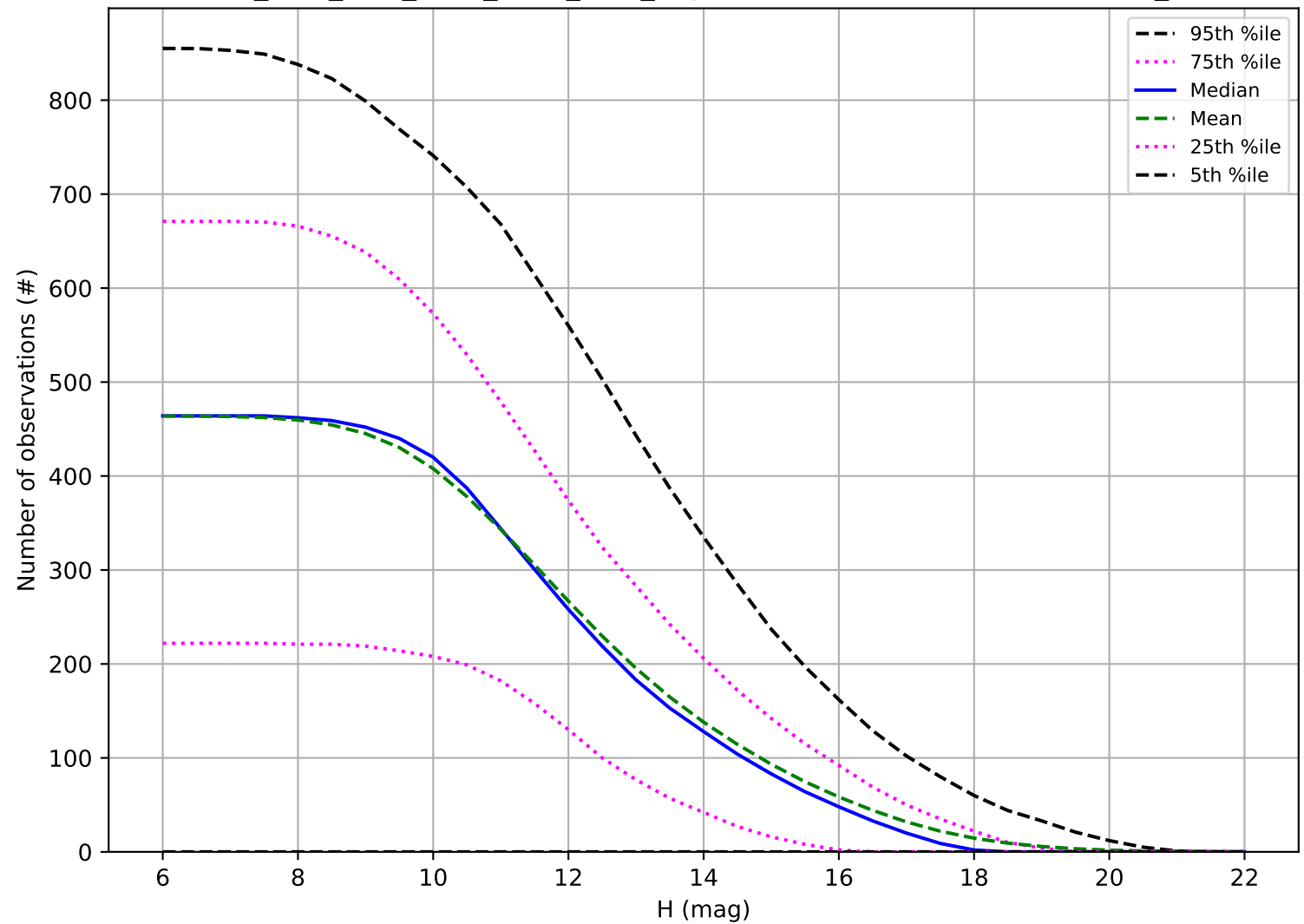
ddf_acor_sf10_lsf15_lsr50_v3.4_10yrs: Number of observations OCC_r5
