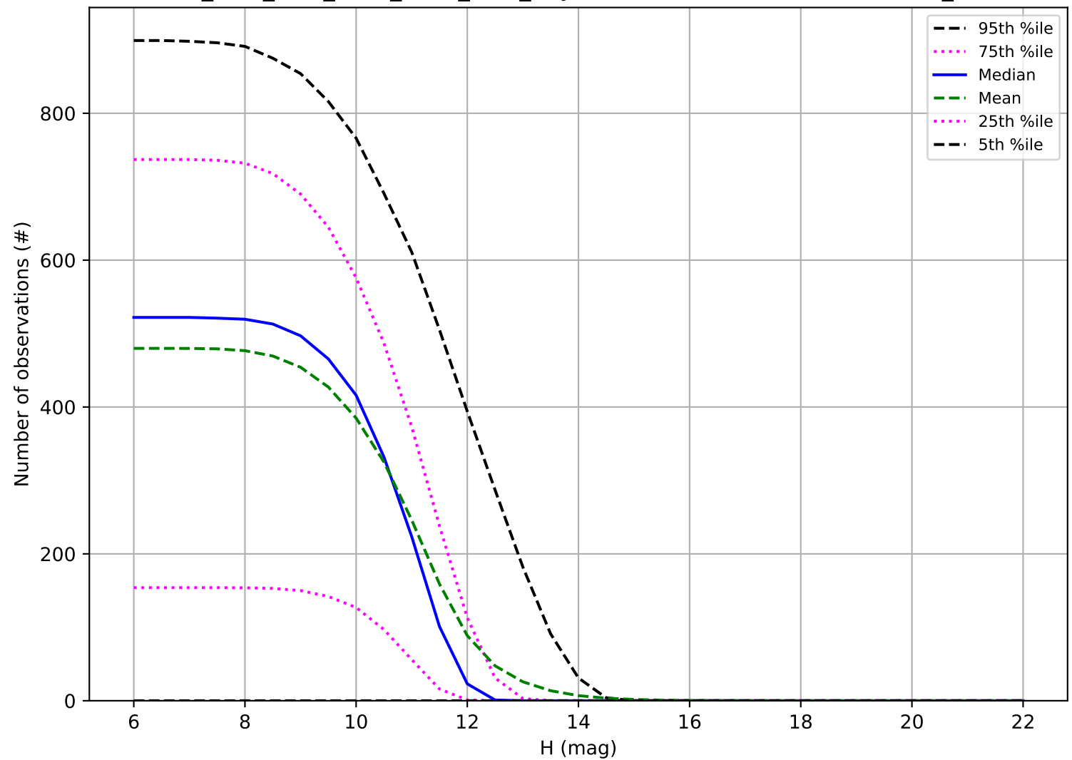
ddf_acor_sf10_lsf15_lsr50_v3.4_10yrs: Number of observations OCC_r20
