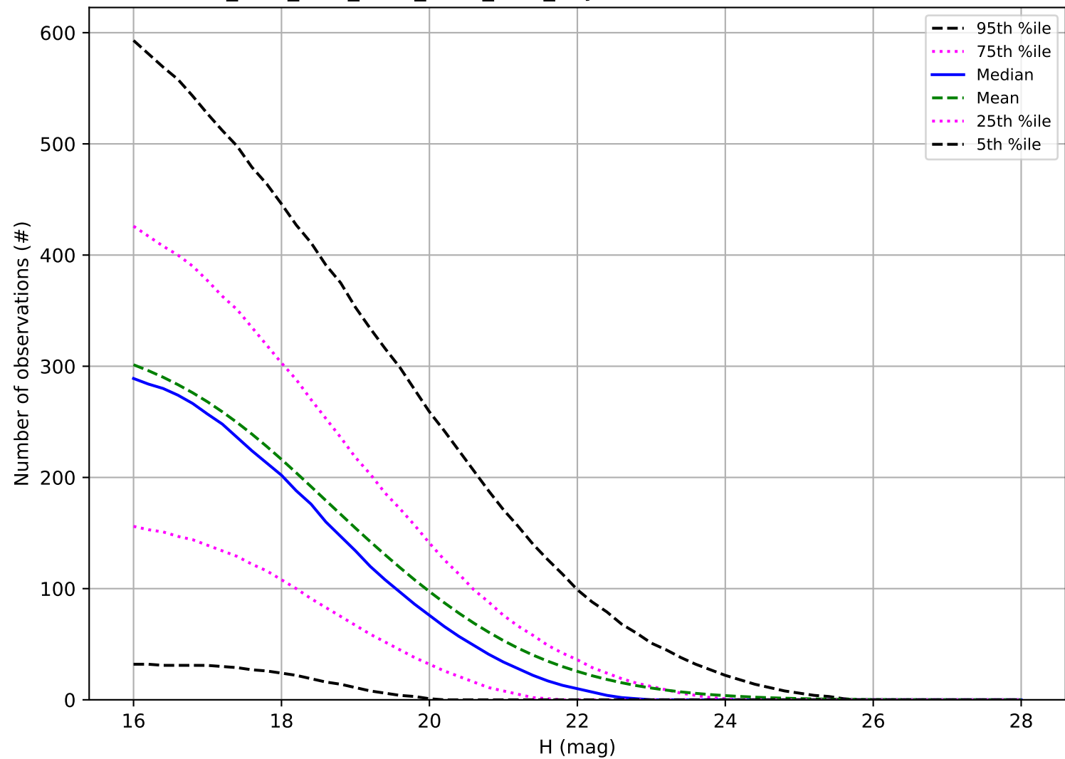
ddf_acor_sf10_lsf15_lsr50_v3.4_10yrs: Number of observations NEO
