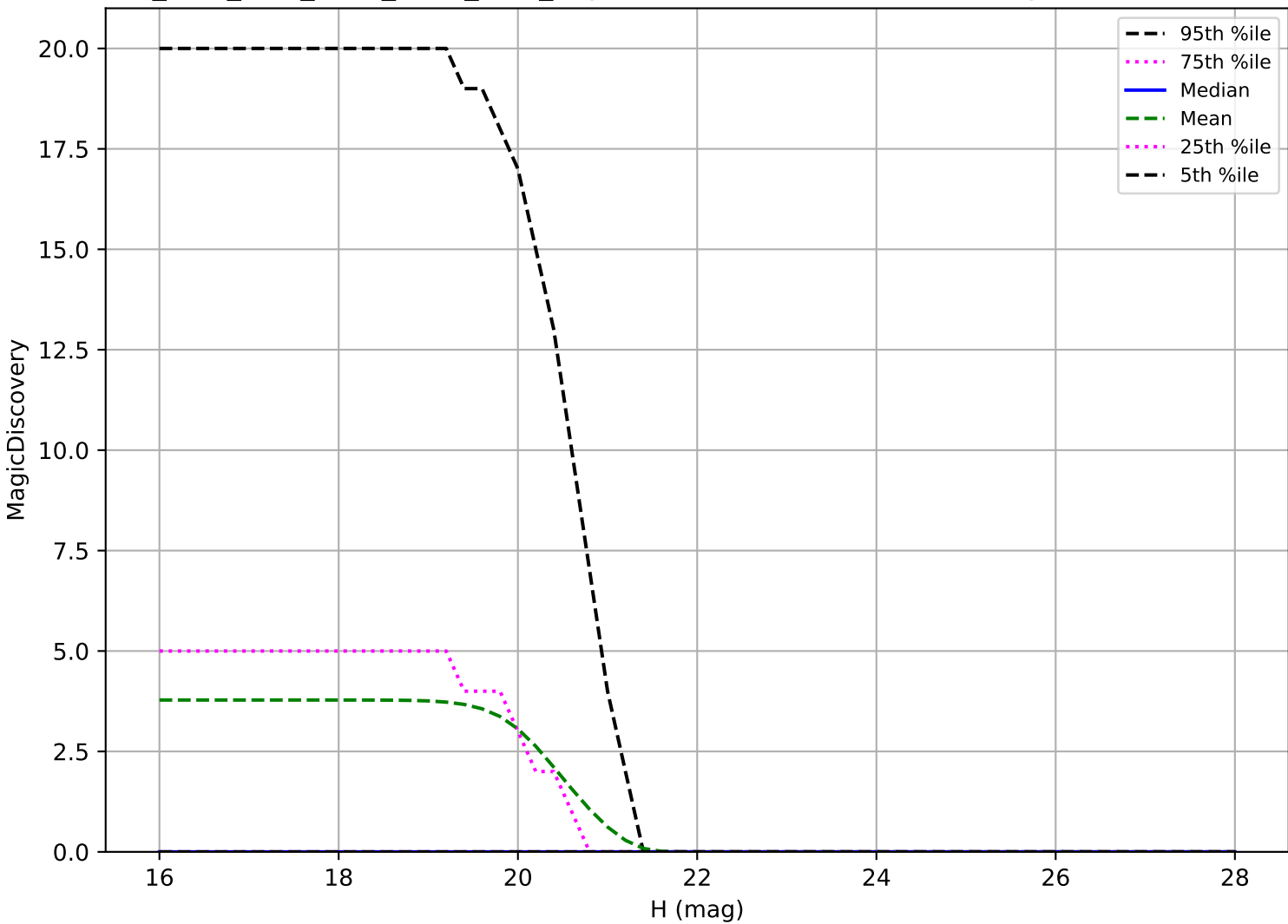
ddf_acor_sf10_lsf15_lsr50_v3.4_10yrs: Vatra 6 detections in 60 nights detection loss
