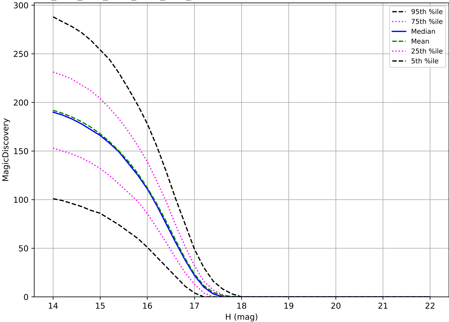
ddf_acor_sf10_lsf15_lsr50_v3.4_10yrs: Trojan 6 detections in 60 nights detection loss
