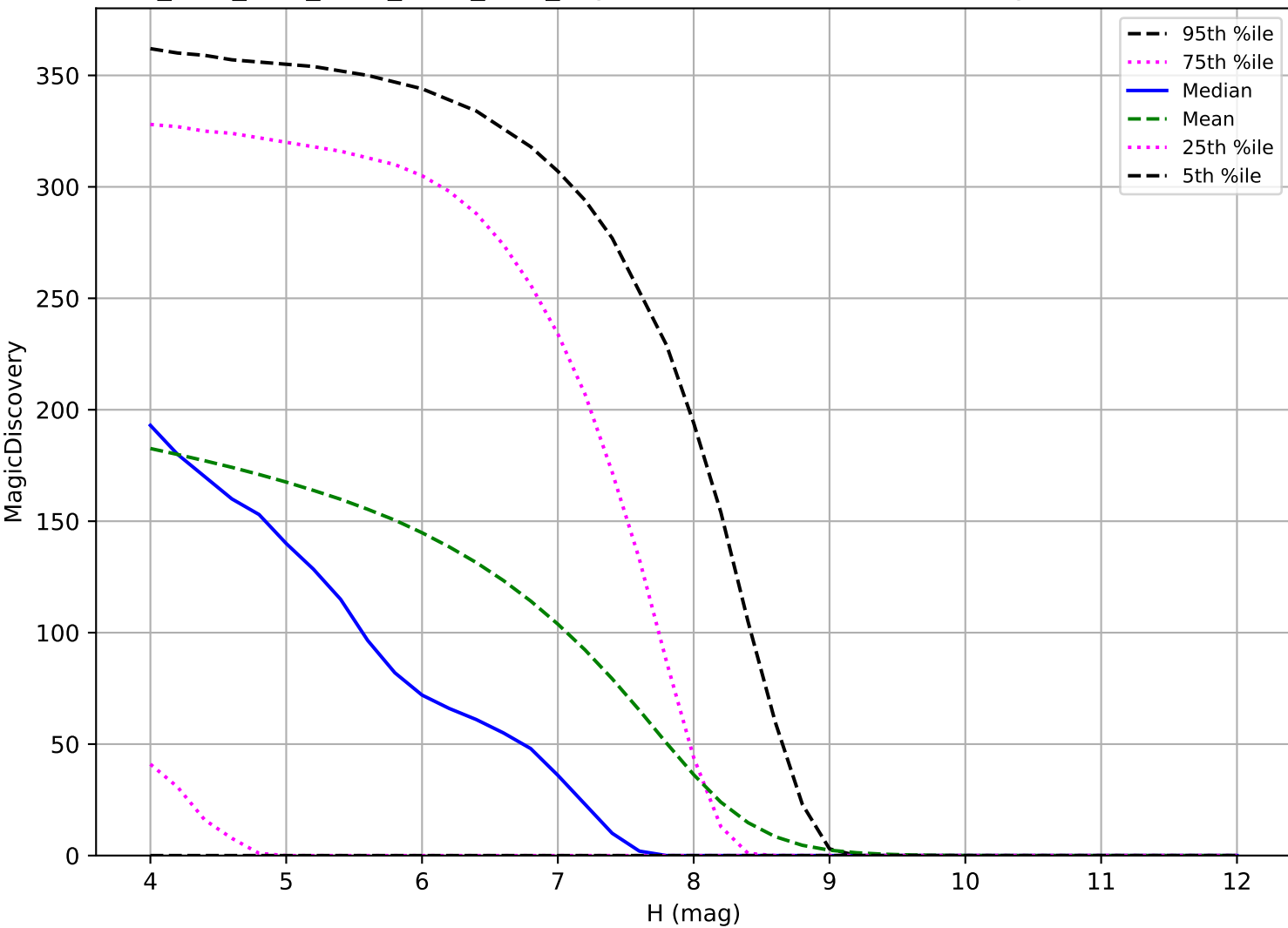
ddf_acor_sf10_lsf15_lsr50_v3.4_10yrs: TNO 6 detections in 60 nights detection loss
