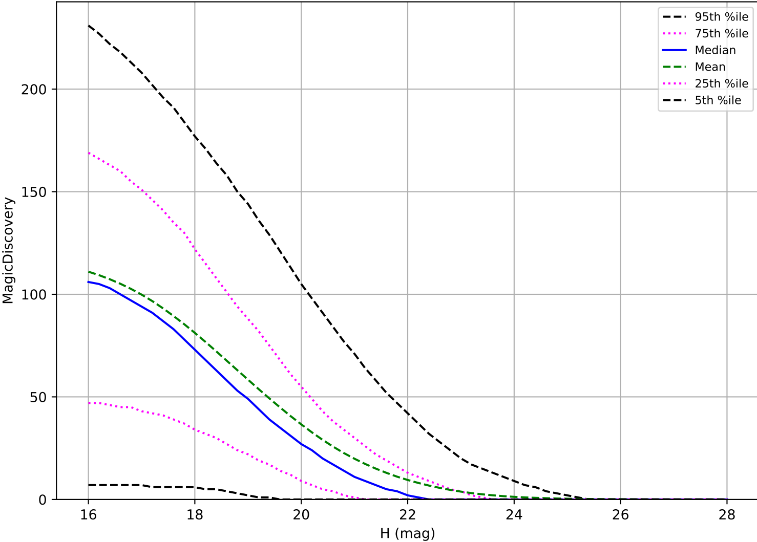
ddf_acor_sf10_lsf15_lsr50_v3.4_10yrs: PHA 6 detections in 60 nights detection loss
