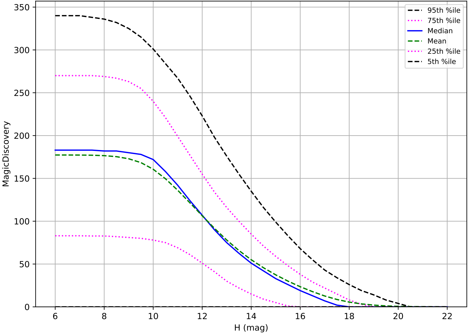
ddf_acor_sf10_lsf15_lsr50_v3.4_10yrs: OCC_r5 6 detections in 60 nights detection loss
