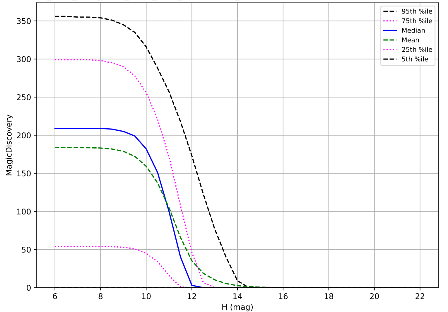
ddf_acor_sf10_lsf15_lsr50_v3.4_10yrs: OCC_r20 6 detections in 60 nights detection loss
