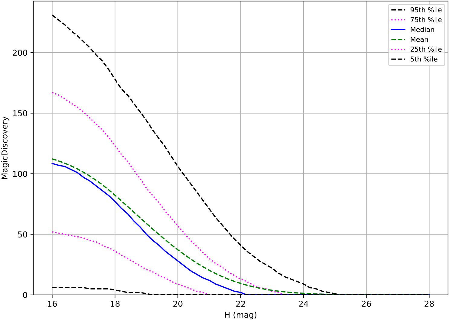
ddf_acor_sf10_lsf15_lsr50_v3.4_10yrs: NEO 6 detections in 60 nights detection loss
