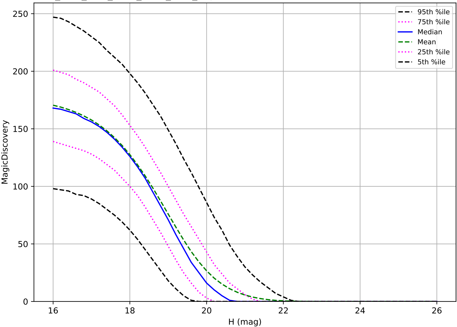
ddf_acor_sf10_lsf15_lsr50_v3.4_10yrs: MBA 6 detections in 60 nights detection loss
