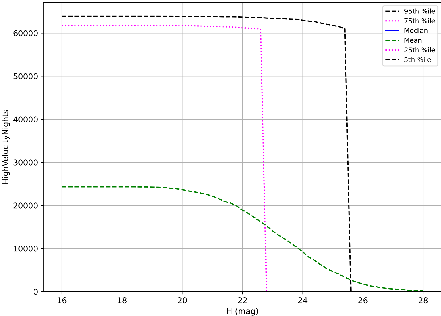
ddf_acor_sf10_lsf15_lsr50_v3.4_10yrs: PHA High velocity pair detection loss
