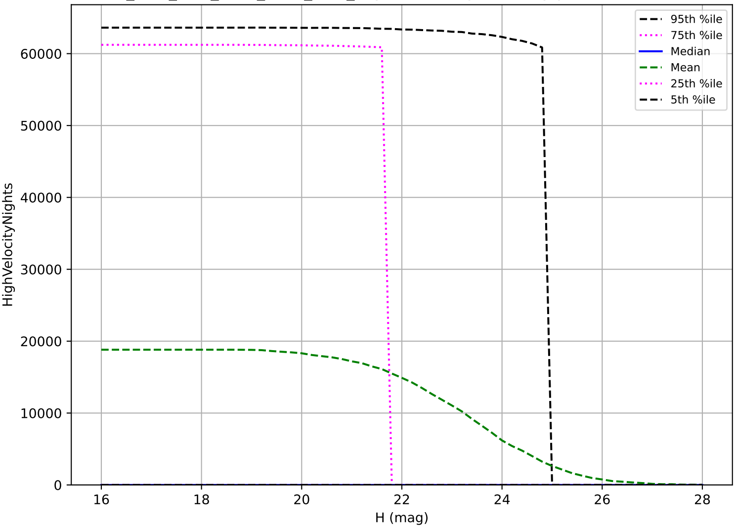
ddf_acor_sf10_lsf15_lsr50_v3.4_10yrs: NEO High velocity pair detection loss
