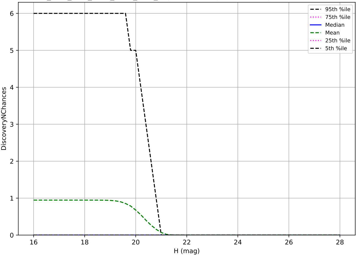
ddf_acor_sf10_lsf15_lsr50_v3.4_10yrs: Vatira 3 pairs in 15 nights detection loss
