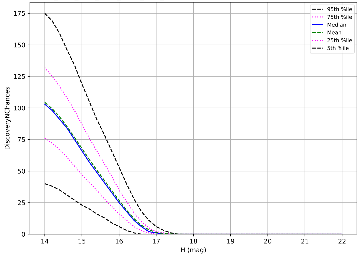
ddf_acor_sf10_lsf15_lsr50_v3.4_10yrs: Trojan 3 pairs in 15 nights detection loss
