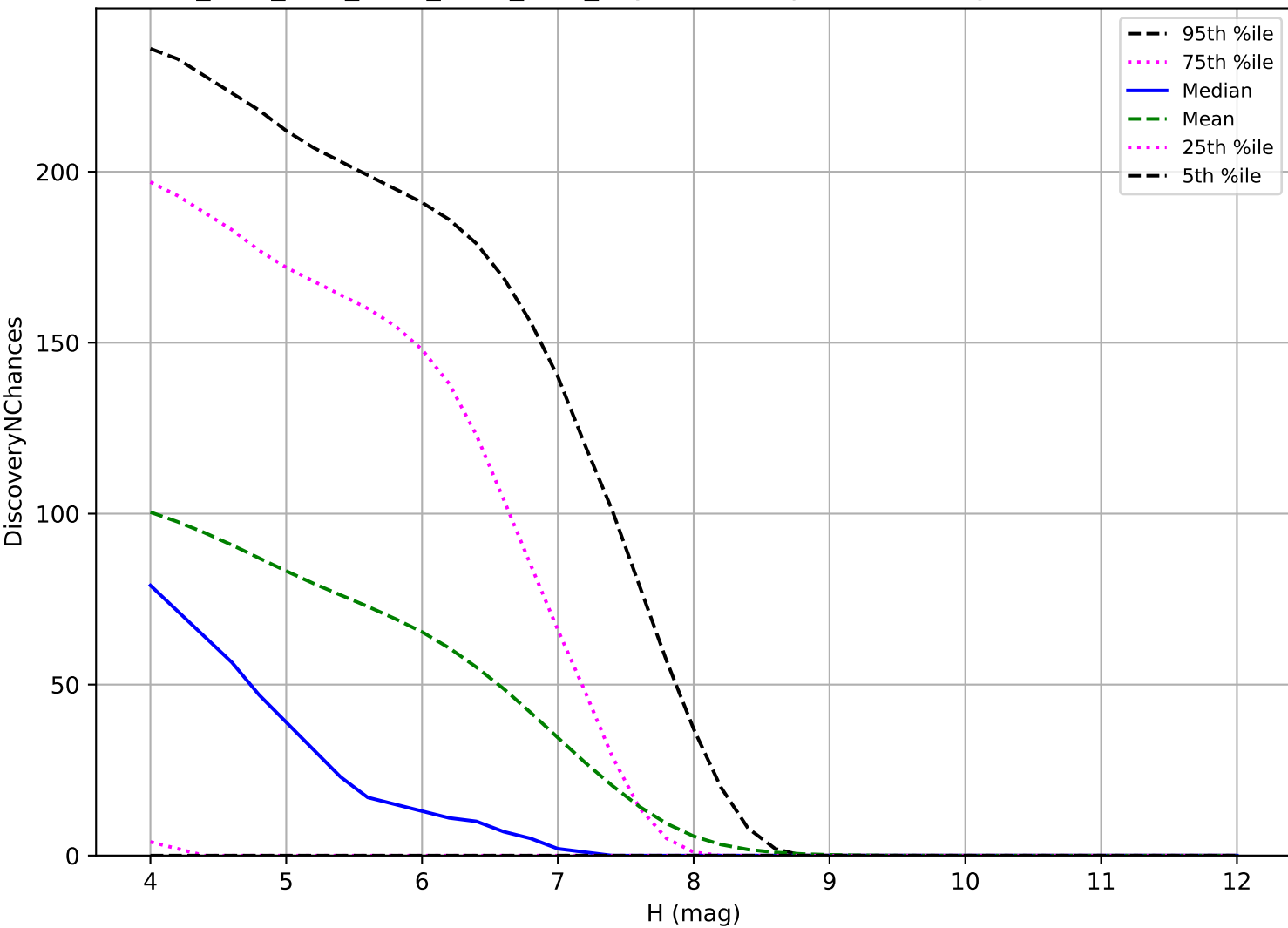
ddf_acor_sf10_lsf15_lsr50_v3.4_10yrs: TNO 3 pairs in 15 nights detection loss
