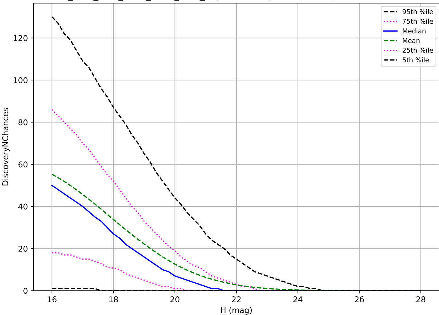
ddf_acor_sf10_lsf15_lsr50_v3.4_10yrs: PHA 3 pairs in 15 nights detection loss
