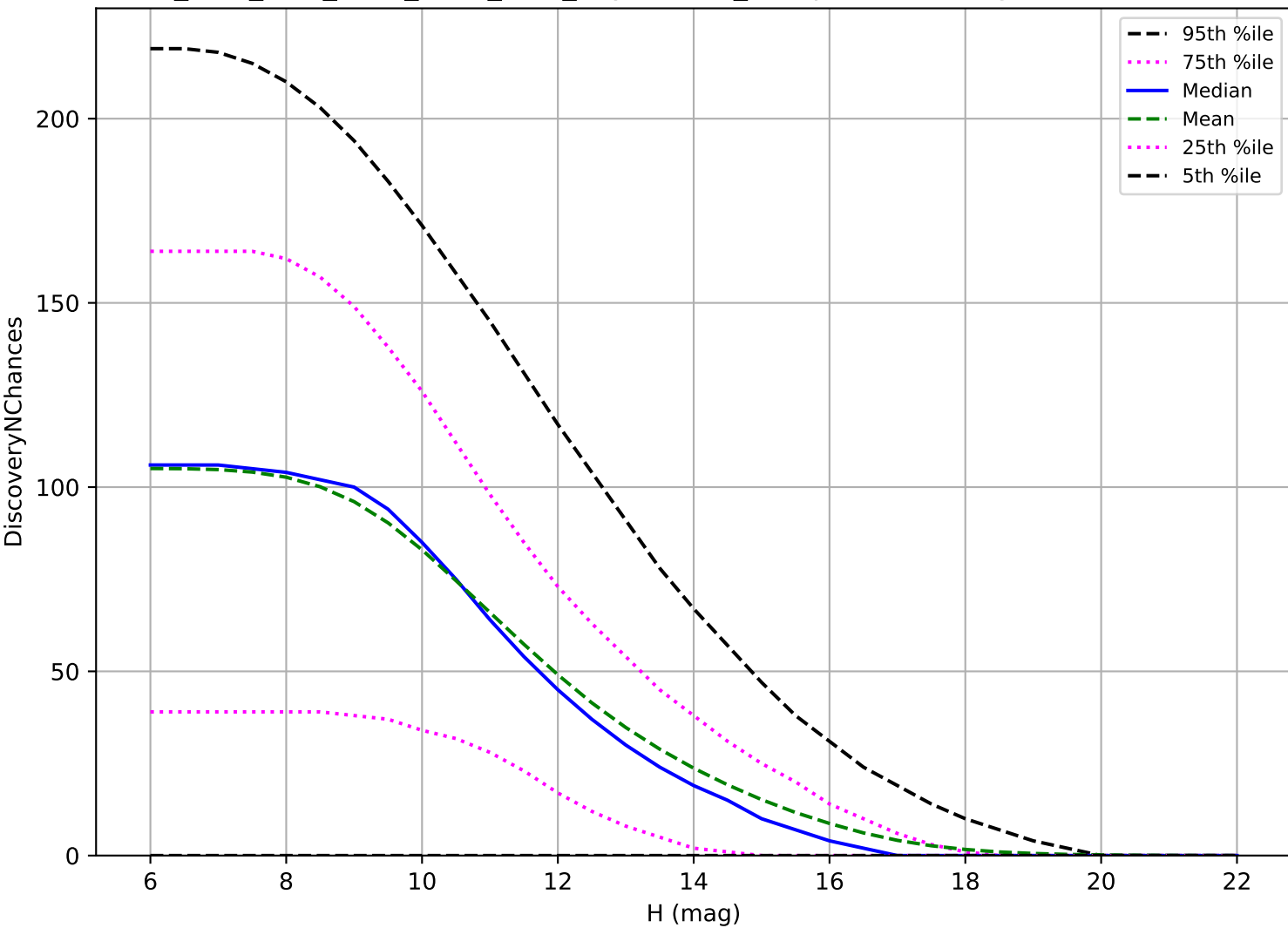
ddf_acor_sf10_lsf15_lsr50_v3.4_10yrs: OCC_r5 3 pairs in 15 nights detection loss
