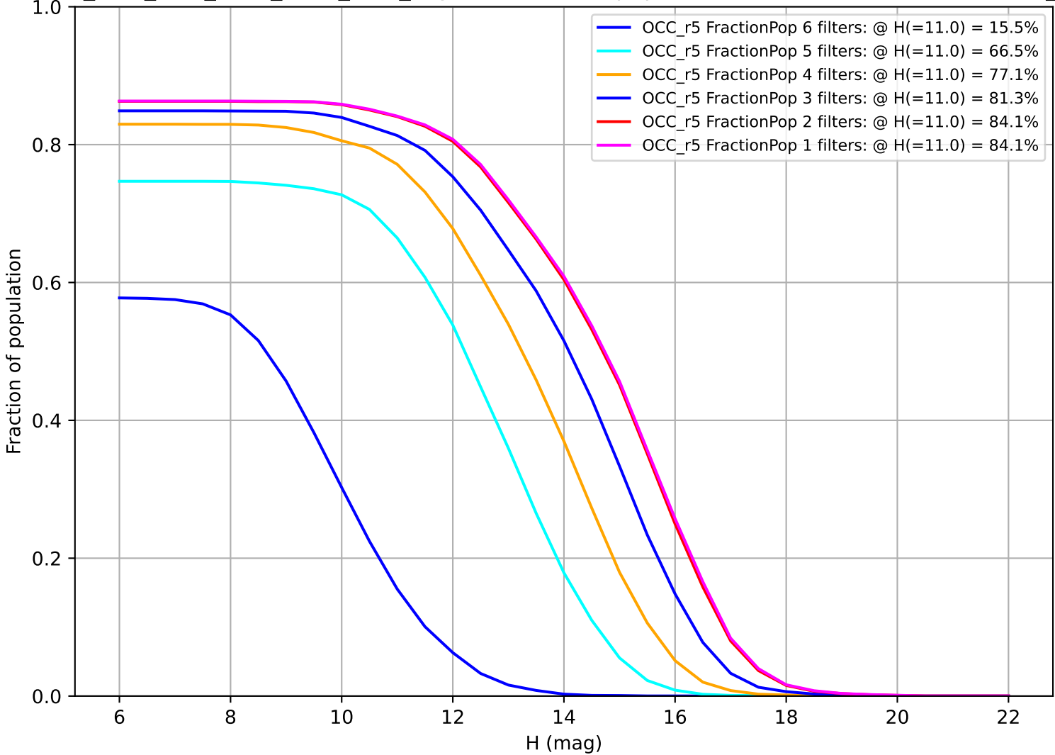
ddf_acor_sf10_lsf15_lsr50_v3.4_10yrs: Fraction of population with colors in X filters OCC_r5
