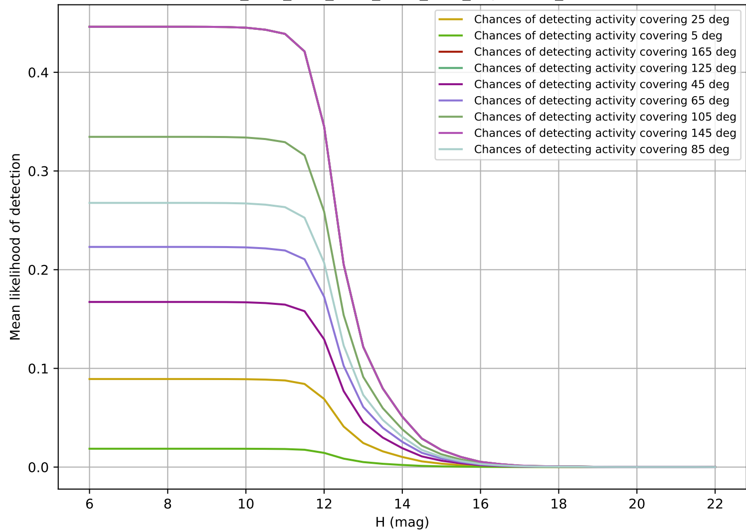
ddf_acor_sf10_lsf15_lsr50_v3.4_10yrs OCC_r20
