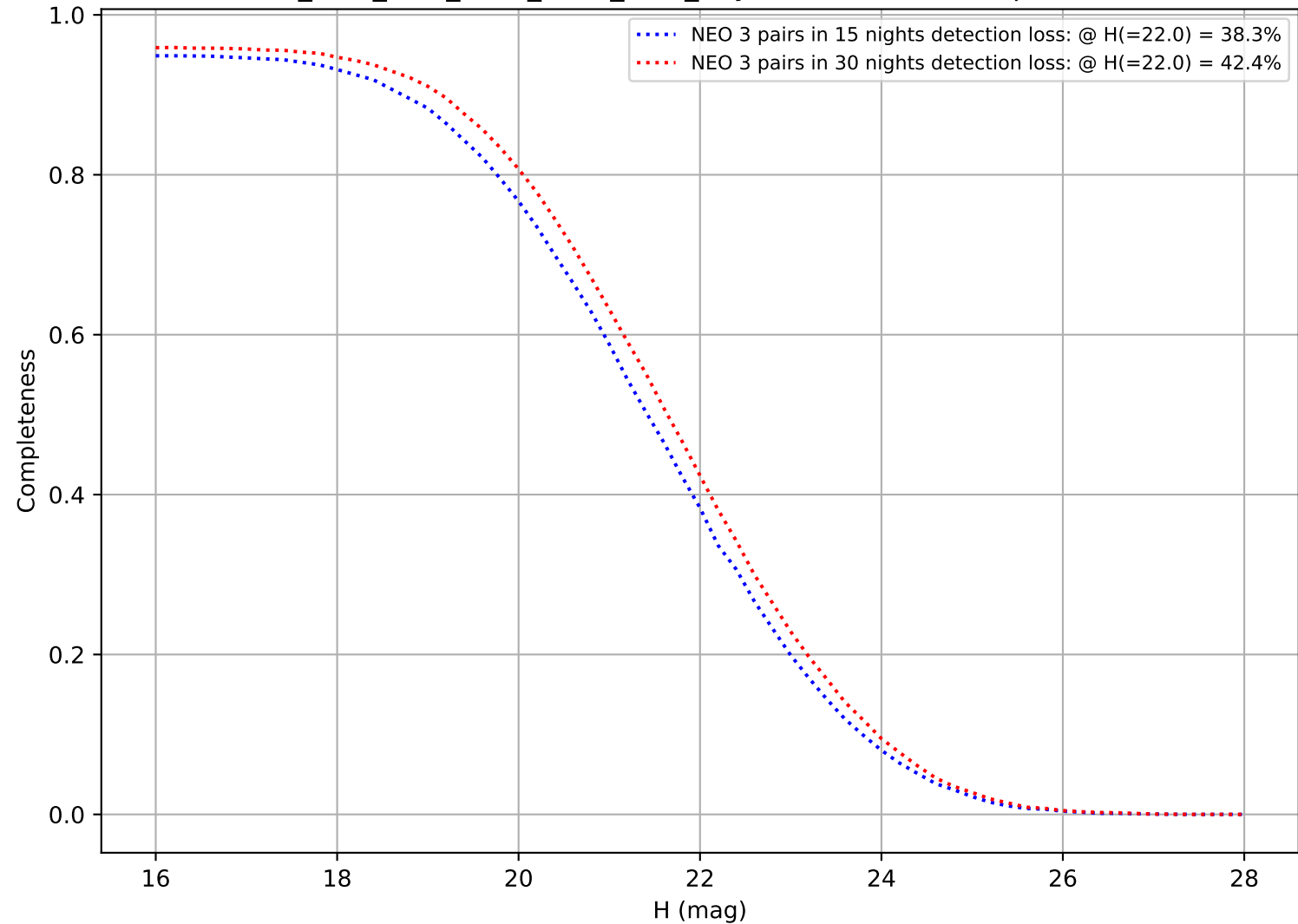
ddf_acor_sf10_lsf15_lsr50_v3.4_10yrs: DifferentialCompleteness
