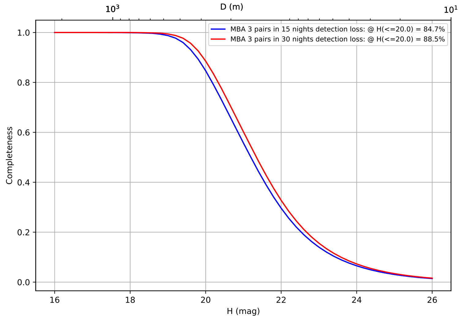
ddf_acor_sf10_lsf15_lsr50_v3.4_10yrs: CumulativeCompleteness
