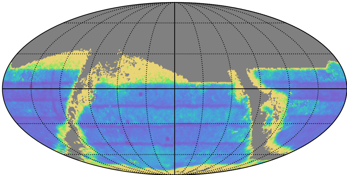
ddf_acor_sf10_lsf15_lsr50_v3.4_10yrs : TDC_precision
