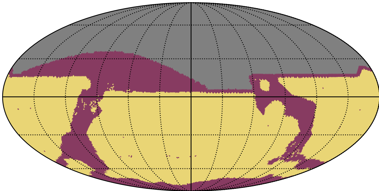
ddf_acor_sf10_lsf15_lsr50_v3.4_10yrs : RapidRevisits
