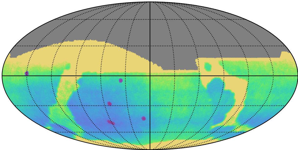
ddf_acor_sf10_lsf15_lsr50_v3.4_10yrs : Parallax Uncert @ 24.0
