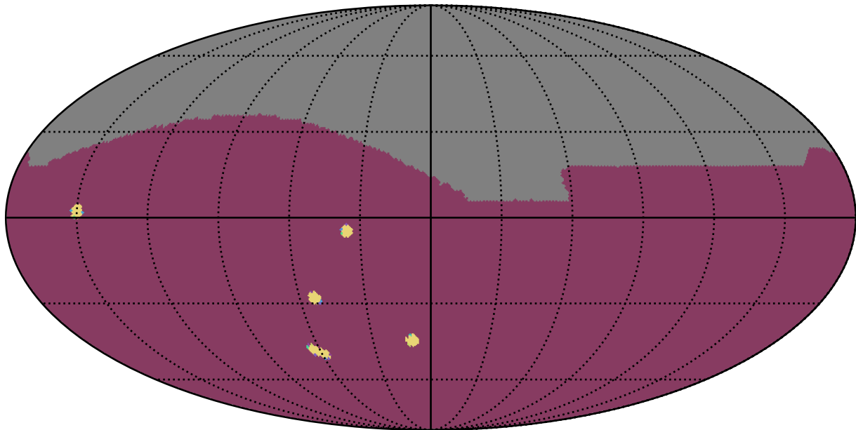
ddf_acor_sf10_lsf15_lsr50_v3.4_10yrs : NumberOfQuickRevisits
