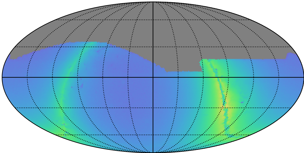
ddf_acor_sf10_lsf15_lsr50_v3.4_10yrs r: Nstars_no_crowding
