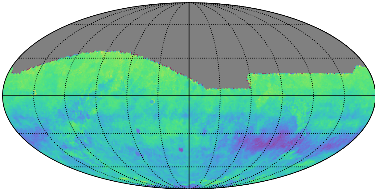
ddf_acor_sf10_lsf15_lsr50_v3.4_10yrs r: Kuiper rotSkyPos
