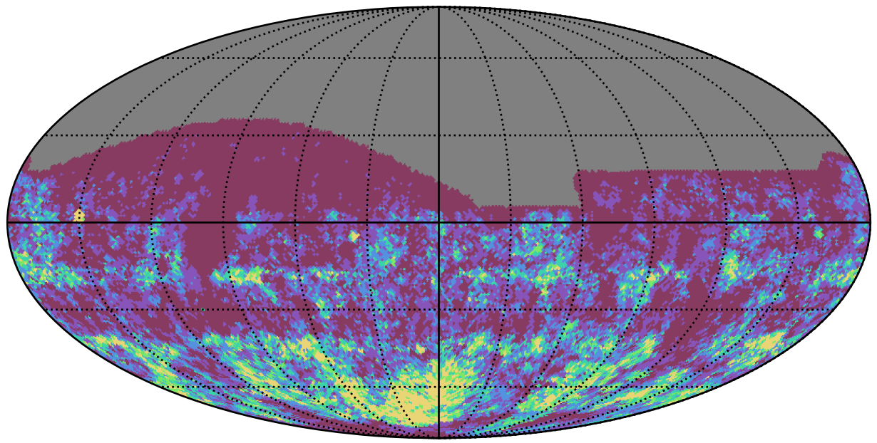
ddf_acor_sf10_lsf15_lsr50_v3.4_10yrs r band: Gaps_3hr
