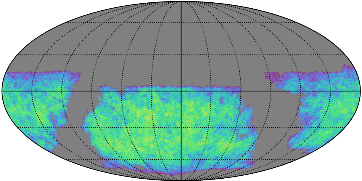
ddf_acor_sf10_lsf15_lsr50_v3.4_10yrs i band non-DD year 1: ExgalM5WithCuts
