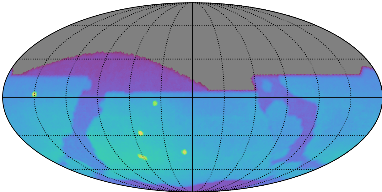
ddf_acor_sf10_lsf15_lsr50_v3.4_10yrs : Brown Dwarf, L4
