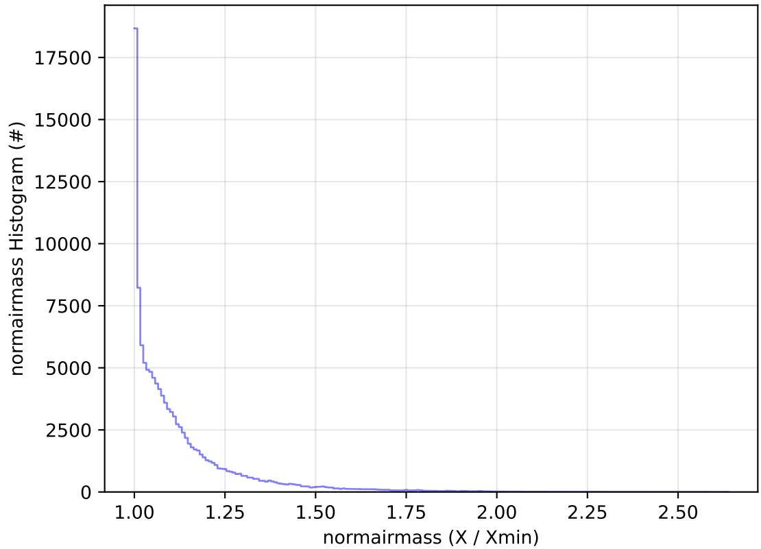
ddf_acor_sf10_lsf15_lsr50_v3.4_10yrs All sky u band: normairmass Histogram
