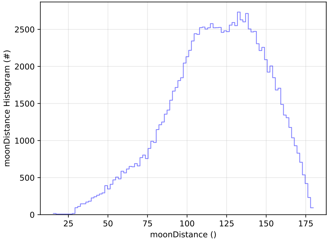
ddf_acor_sf10_ls15_lsr50_v3.4_10yrs WFD u band: moonDistance Histogram
