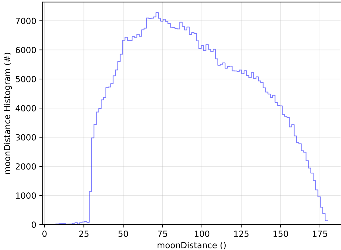
ddf_acor_sf10_lsf15_lsr50_v3.4_10yrs All sky i band: moonDistance Histogram
