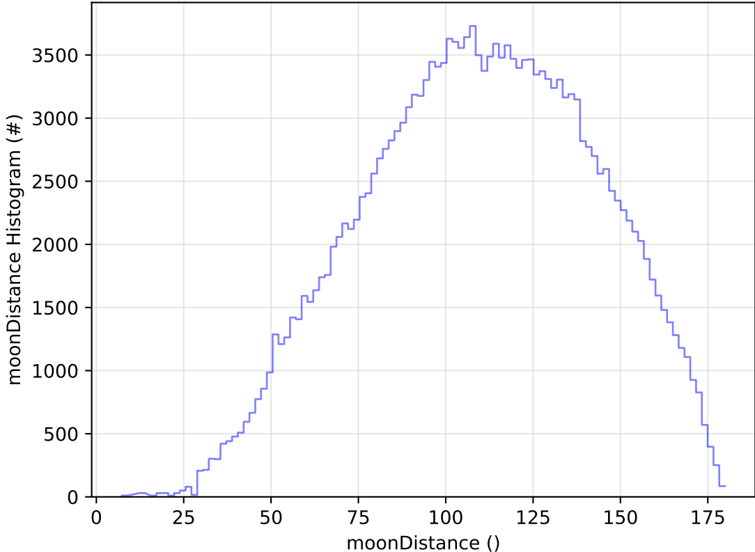
ddf_acor_sf10_lsf15_lsr50_v3.4_10yrs All sky g band: moonDistance Histogram
