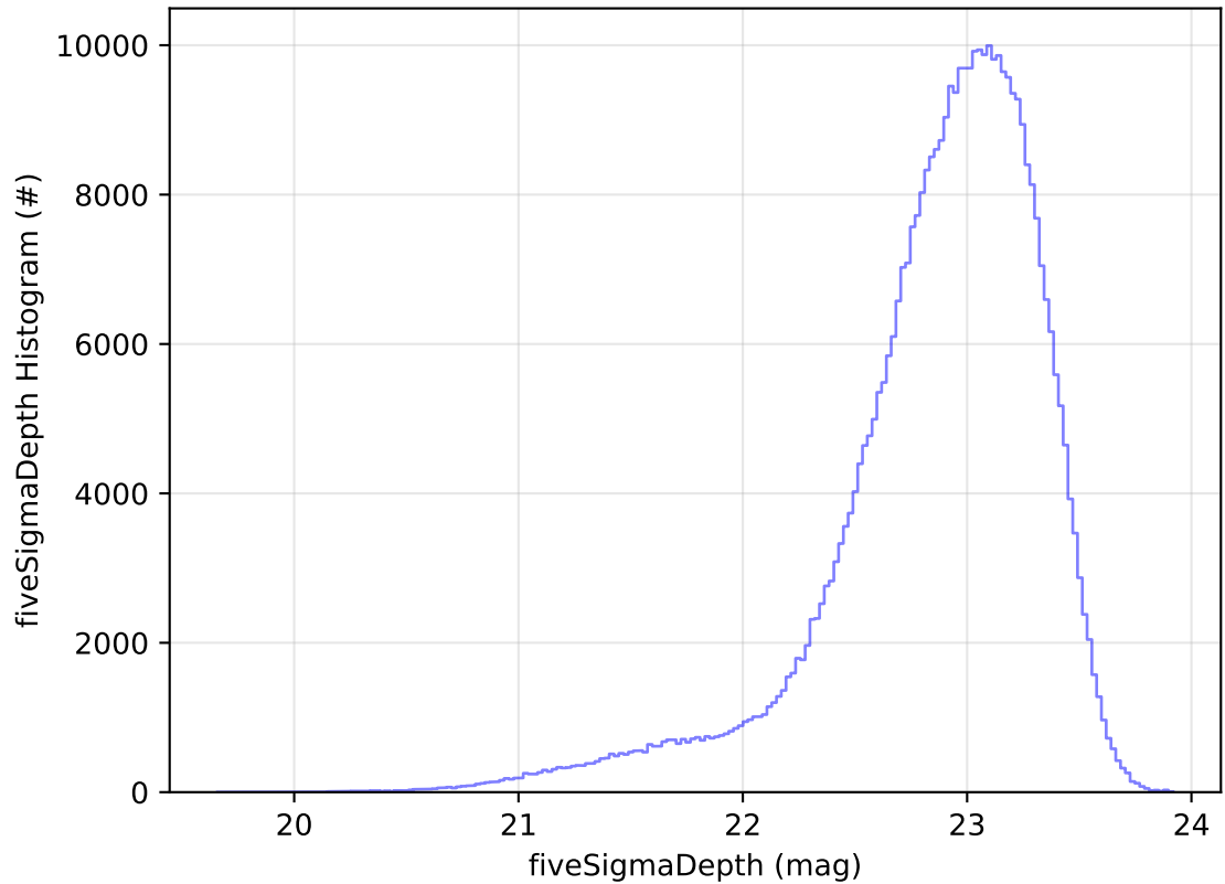
ddf_acor_sf10_ls15_lsr50_v3.4_10yrs WFD z band: fiveSigmaDepth Histogram
