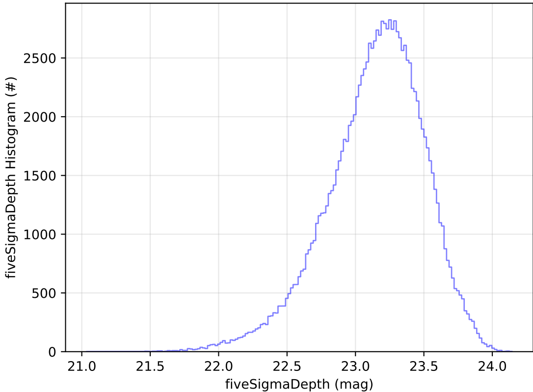
ddf_acor_sf10_lsf15_lsr50_v3.4_10yrs WFD u band: fiveSigmaDepth Histogram
