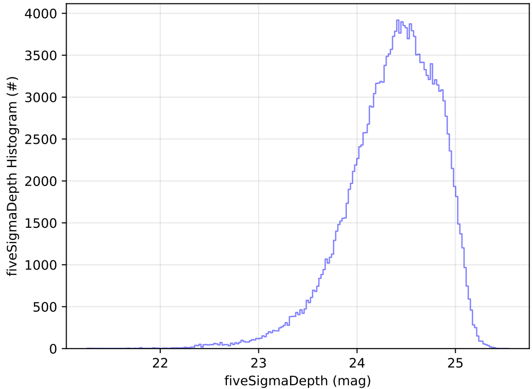
ddf_acor_sf10_lsf15_lsr50_v3.4_10yrs WFD g band: fiveSigmaDepth Histogram
