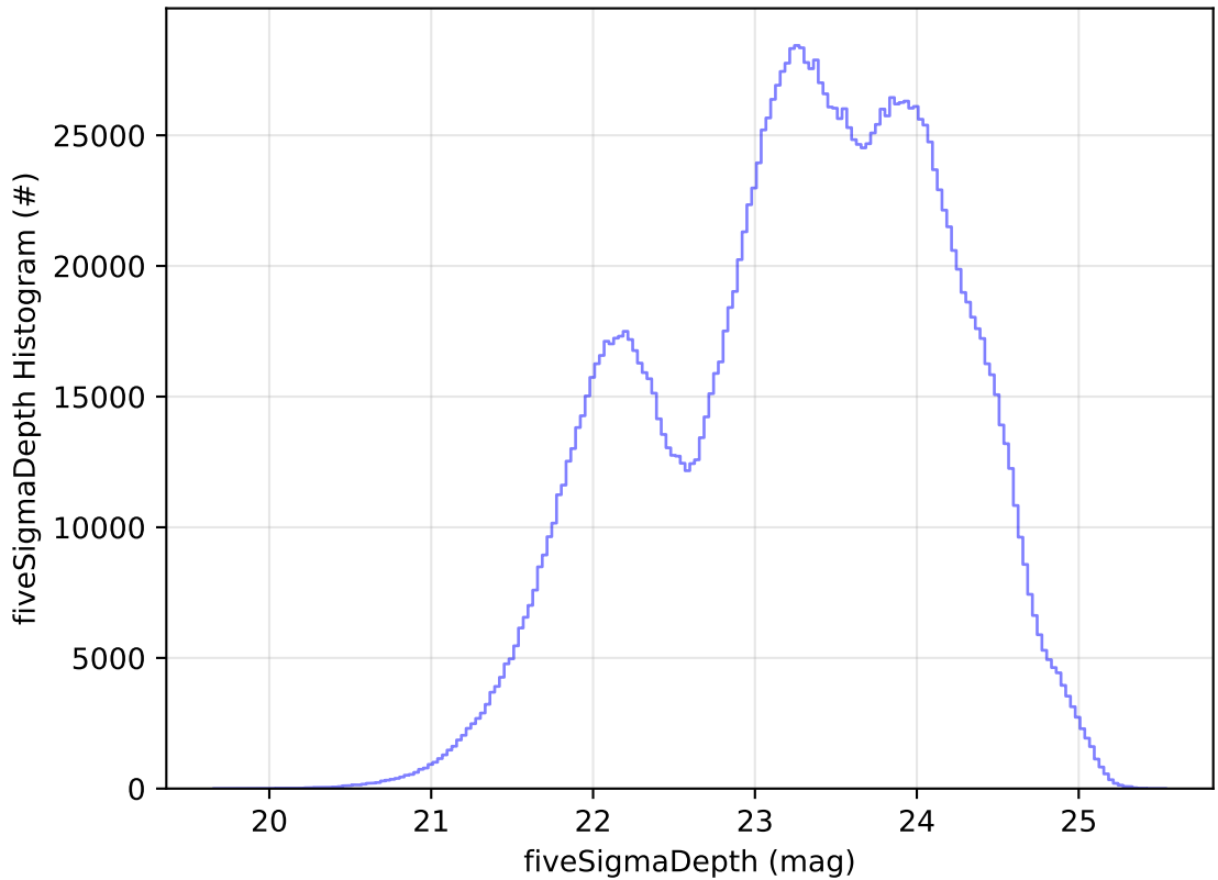
ddf_acor_sf10_lsf15_lsr50_v3.4_10yrs WFD all bands: fiveSigmaDepth Histogram
