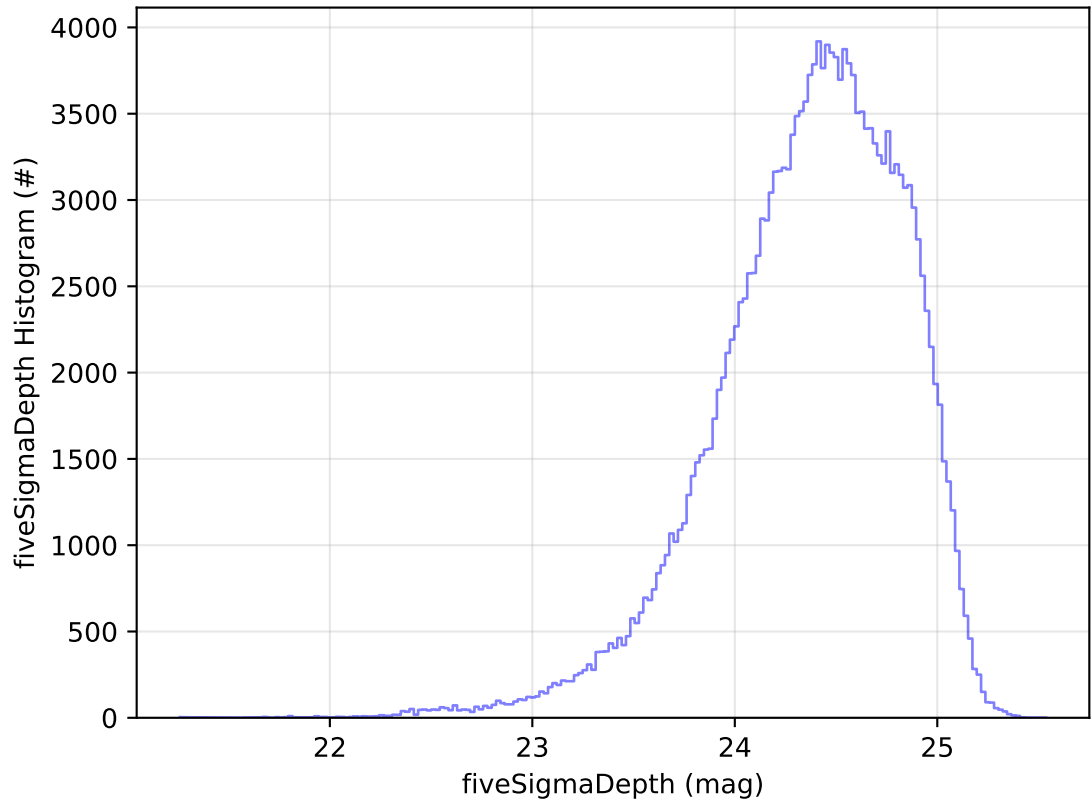
ddf_acor_sf10_lsf15_lsr50_v3.4_10yrs All sky g band: fiveSigmaDepth Histogram
