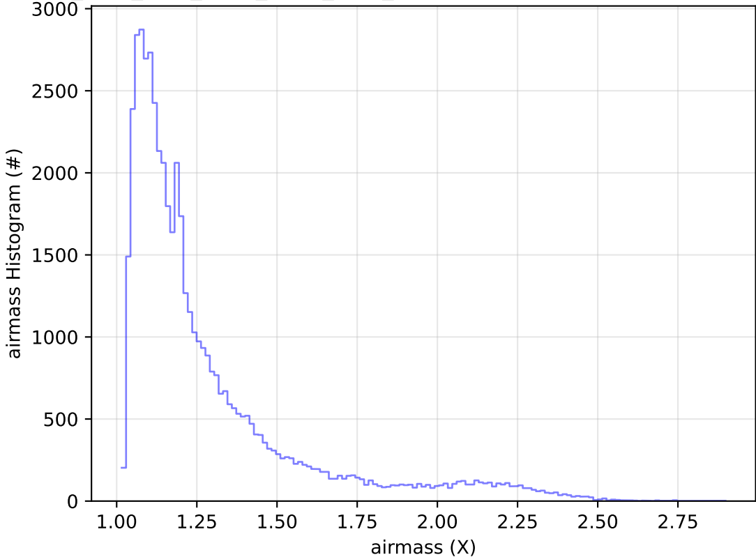
ddf_acor_sf10_lsf15_lsr50_v3.4_10yrs Yr 1 r band: airmass Histogram
