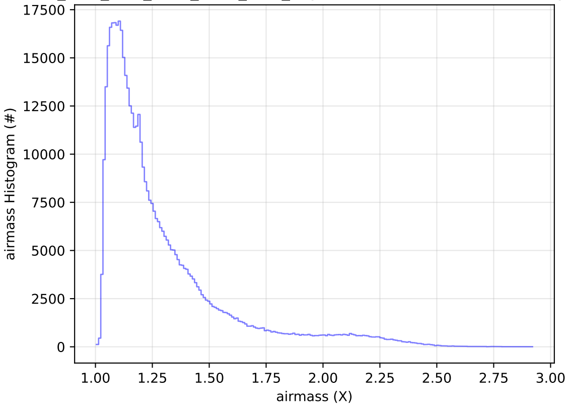
ddf_acor_sf10_lsf15_lsr50_v3.4_10yrs WFD r band: airmass Histogram
