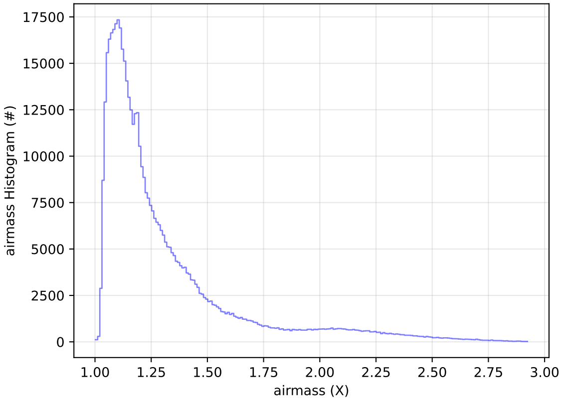
ddf_acor_sf10_lsf15_lsr50_v3.4_10yrs WFD i band: airmass Histogram
