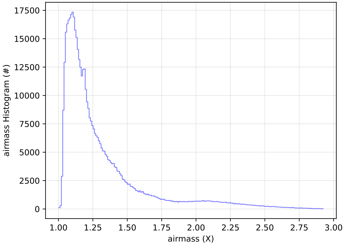
ddf_acor_sf10_lsf15_lsr50_v3.4_10yrs All sky i band: airmass Histogram
