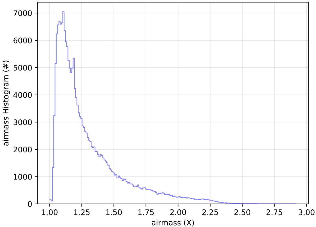
ddf_acor_sf10_lsf15_lsr50_v3.4_10yrs All sky g band: airmass Histogram
