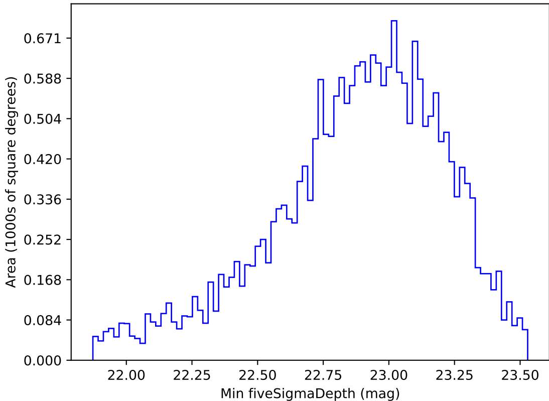
ddf_acor_sf10_lsf15_lsr50_v3.4_10yrs Yr 1 u band: Min fiveSigmaDepth
