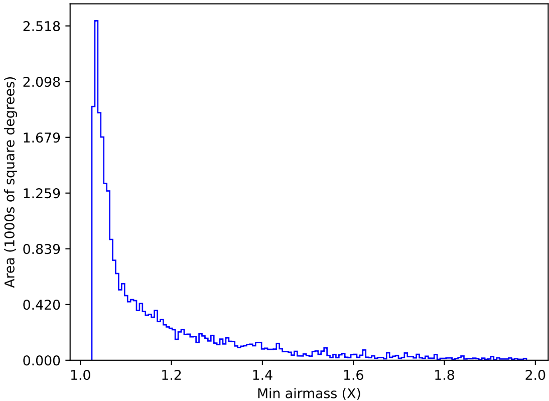
ddf_acor_sf10_lsf15_lsr50_v3.4_10yrs Yr 1 z band: Min airmass
