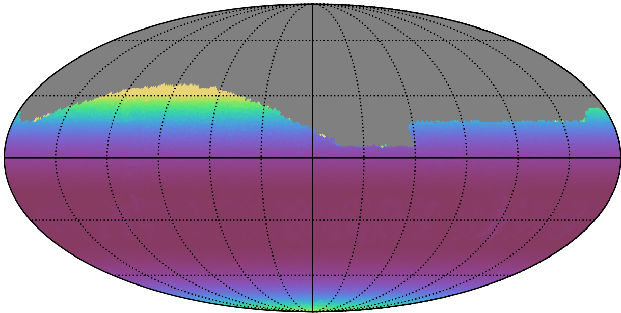
ddf_acor_sf10_lsf15_lsr50_v3.4_10yrs Yr 1 all bands: Min airmass
